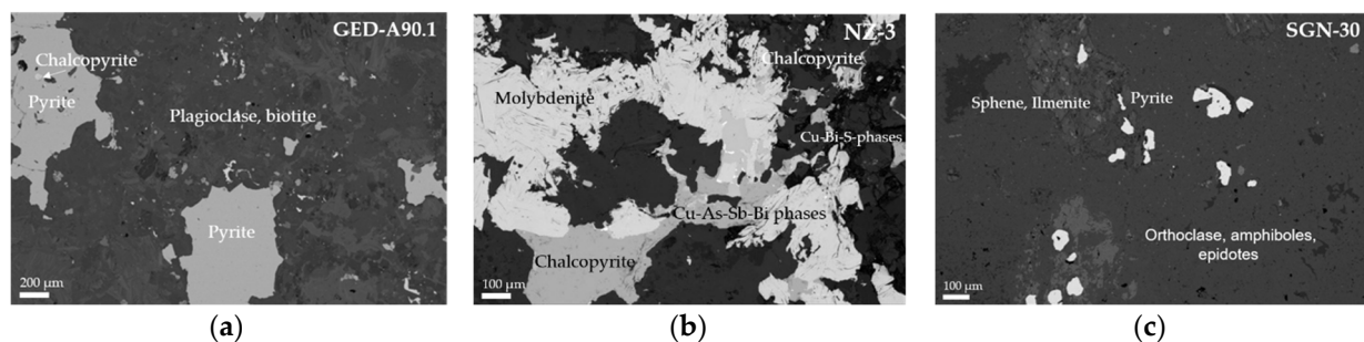
Figure 2. SEM micrographs: (a) GED-A90.1: Pyrite with chalcopyrite (CuFeS 2 ) inclusion; (b) NZ-3: Overview on ore minerals; (c) SGN-30: Pyrite and associated Mo, PbS, Te-Bi phases.
